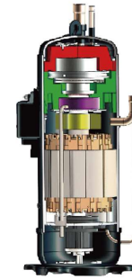
EVI compressor
